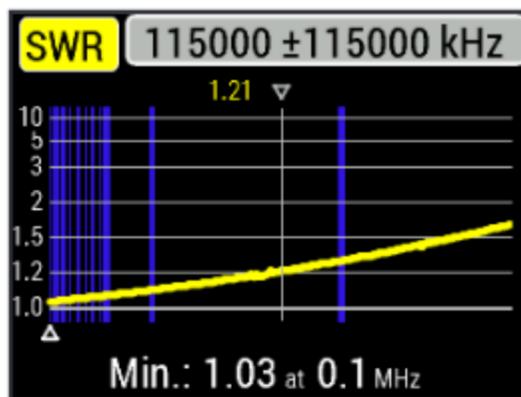
Bird 8201 500 Watt oil-cooled termination High SWR
